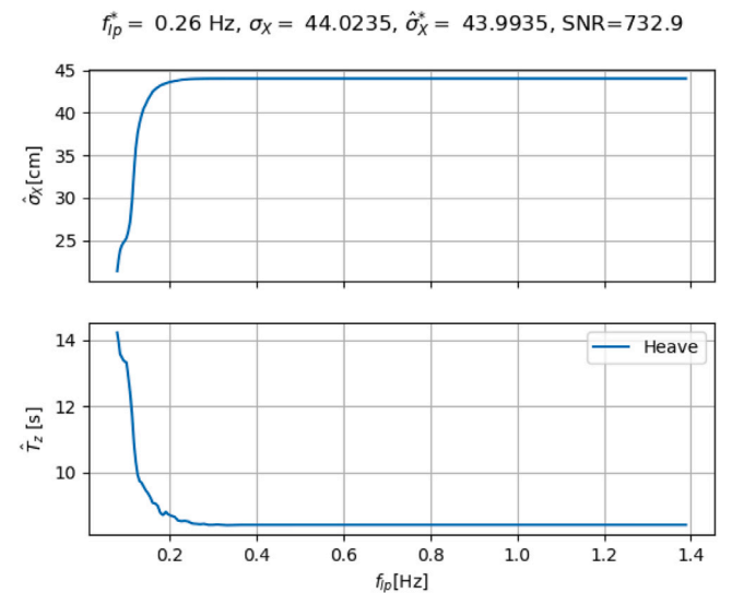
Fig. 14. \hat{\sigma}_X - f_{lp} and \hat{T}_z - f_{lp} curves of heave motion for CaseA1.
