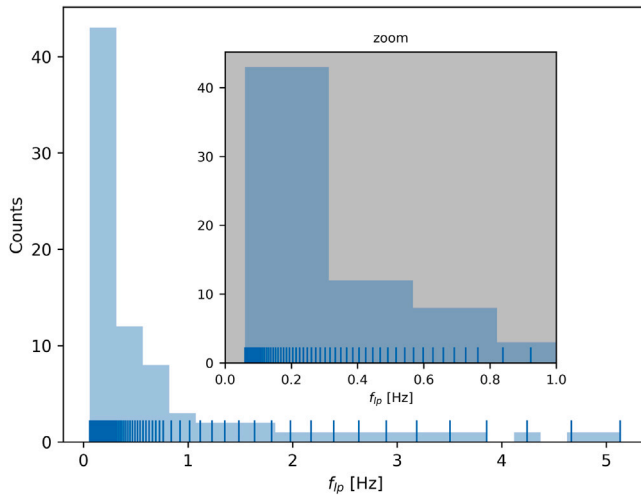
Fig. 12. Histogram of tested f_{lp} values. The blue sticks along the f_{lp} axis represent the data points.
